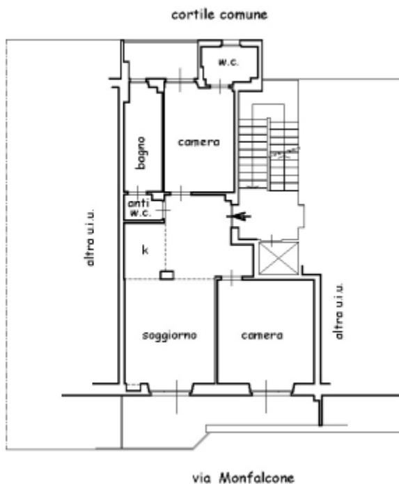
PIANTA PIANO SESTO H = 2.95 mt.
